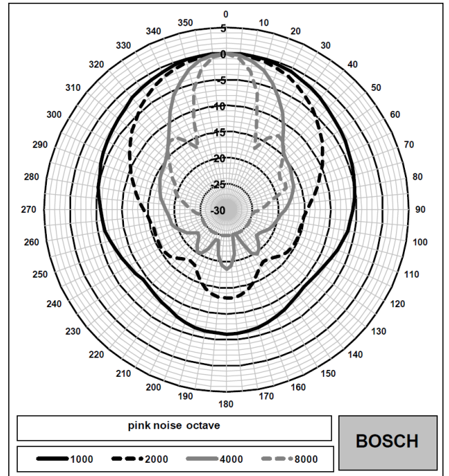
Fig. 7: Vertical polar diagram (high frequency part)
