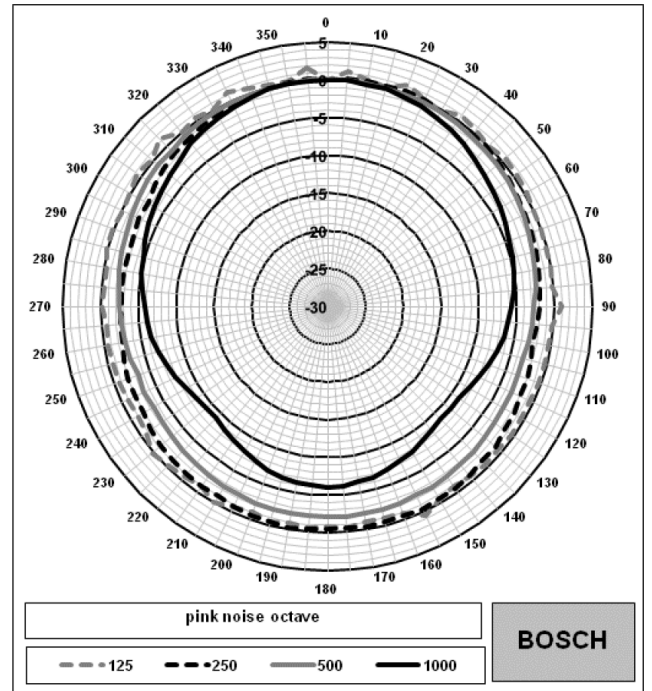
Fig. 6: Vertical polar diagram (low frequency part)
